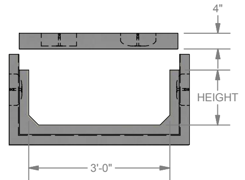
ELEV. VIEW
