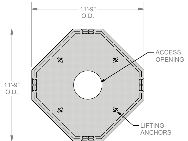
PLAN VIEW (TOP)
