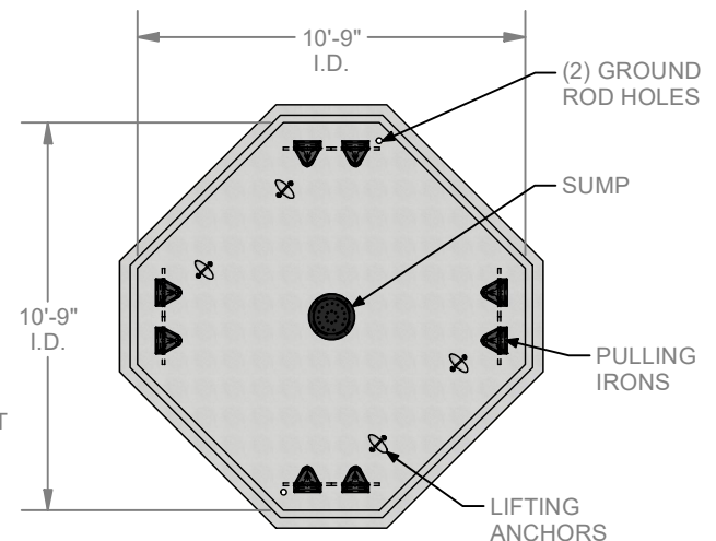
PLAN VIEW (BASE)
