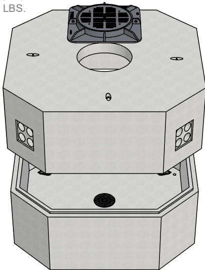
BASE SECTION ~18,500 LBS.
