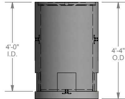
ELEV. VIEW
