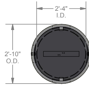
PLAN VIEW (TOP)
