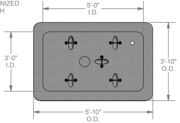
PLAN VIEW (FLOOR)
