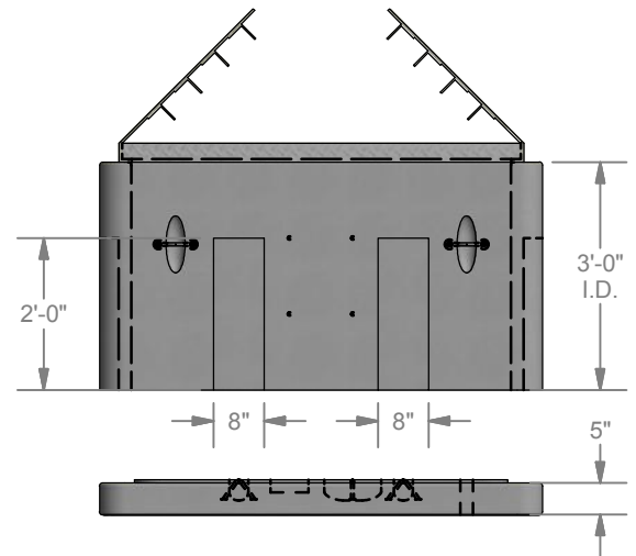
ELEV. VIEW
