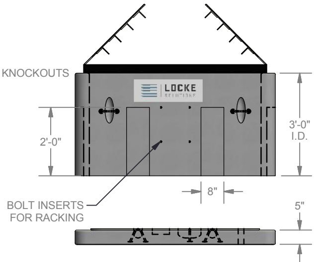
ELEV. VIEW
