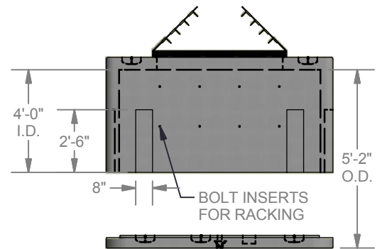
ELEV. VIEW
