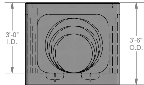
ELEV. VIEW
