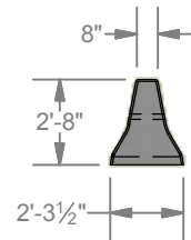
PLAN VIEW (BODY)
