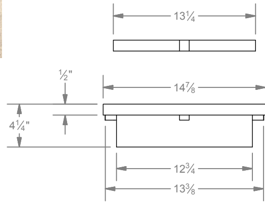
ELEV. VIEW
