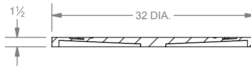
SECTION E-E SCALE 1 / 15
