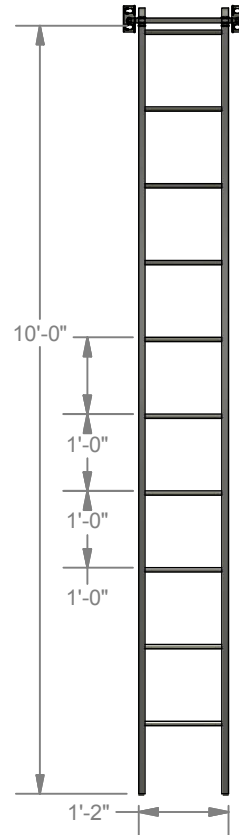
ELEVATION VIEW
