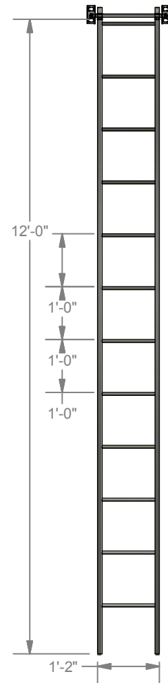
ELEVATION VIEW
