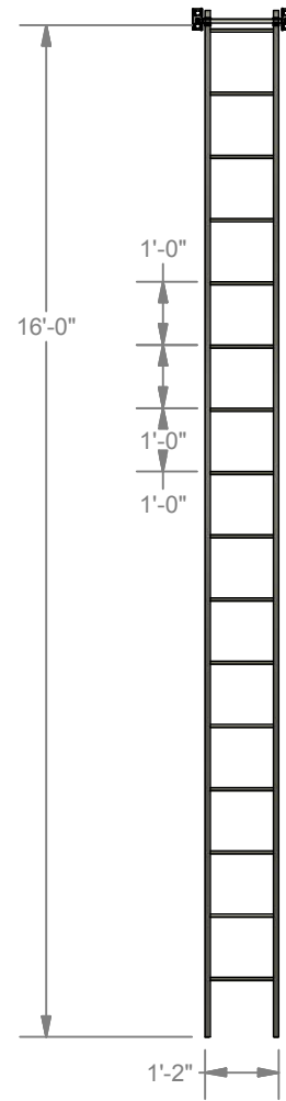
ELEVATION VIEW
