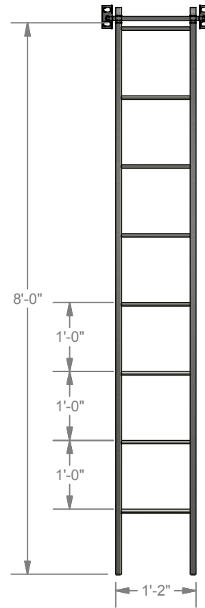
ELEVATION VIEW
