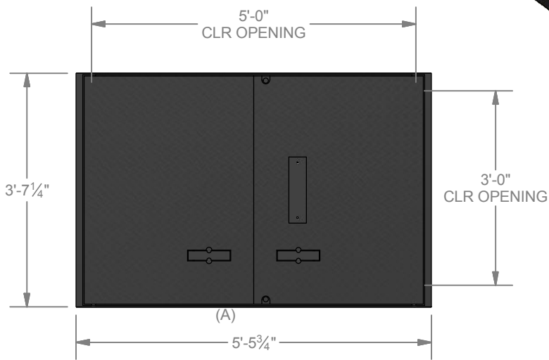
PLAN VIEW (COVER)
