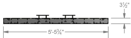
ELEVATION VIEW (A)
