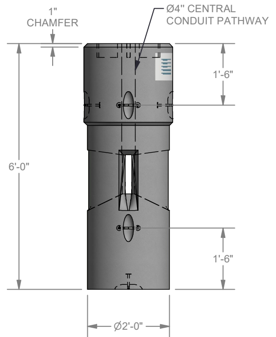
ELEV. VIEW
